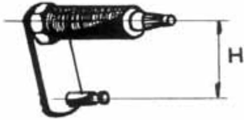
Art. 45.0089 PERNO TERGI H=83mm
