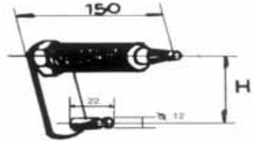
Art. 45.0091 PERNO TERGI H=68,25 mm
