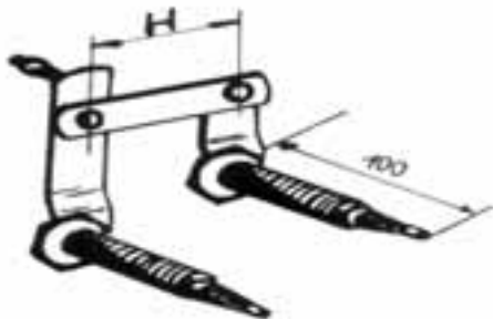
Art. 45.0094 PERNO TANDEM SX H=65 mm
