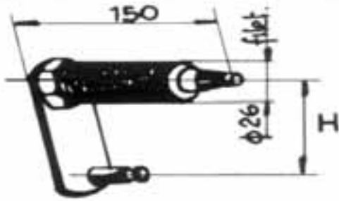
Art. 45.0033 Rif. Orig. 0179126 PERNO TERGI SX H=88 370MN / EURORIDER
