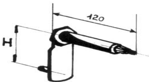
Art. 45.0142 PERNO TERGI H=48mm U210
