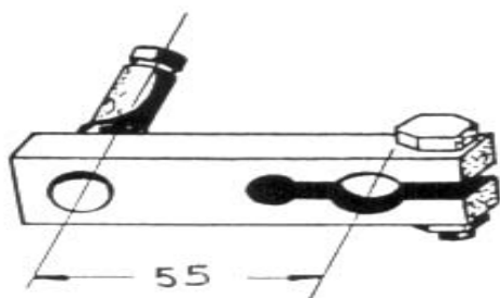
Art. 45.0168 MANOVELLA FORO 11 PERNO 10
