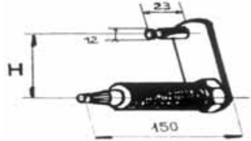
Art. 45.0034 Rif. Orig. 0179127 PERNO TERGI DX H=68,25 370MN / EURORIDER
