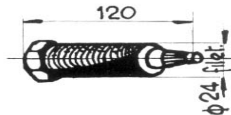
Art. 45.0143 PERNO TERGI L=120mm. U210
